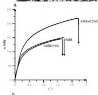
Figure 2. Introduction of nanodiamond particles to an A356 matrix: a, b, OM microstructures showing the distribution of nanoparticles in an A356-0.2 wt% C MMNC; c, tensile curves showing improved strength and ductility at 0.2 wt% addition.
