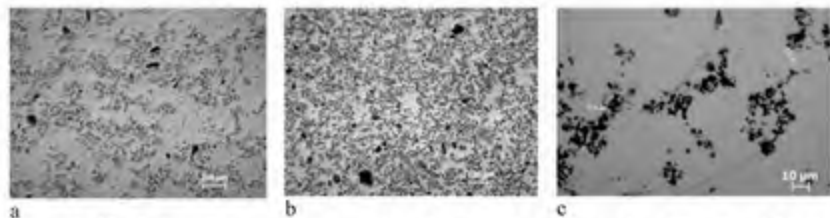
Figure 4. Al-Mg-based composite materials with in-situ formed spinel: a, 1.2 wt% \text{Al}_2\text{MgO}_4 (matrix Al-0.9% Mg-0.5% Si); b, 6 wt% \text{Al}_2\text{MgO}_4 (Al-0.3% Mg-2.2% Si); and c, loose agglomerates with individual spinel particles (OM).
