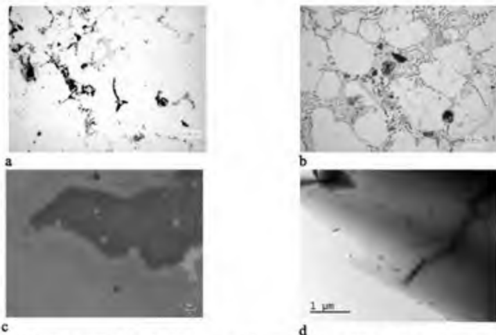
Figure 1. MMNC AA6082-1 wt% \text{Al}_2\text{O}_3 : a, mechanical stirring, OM; b-d, mechanical stirring with ultrasonic processing (b, OM, c, SEM showing particles in agglomerates; d, TEM showing particles in the matrix (courtesy W. Lefebvre, M. Maunib, University of Rouen)).
