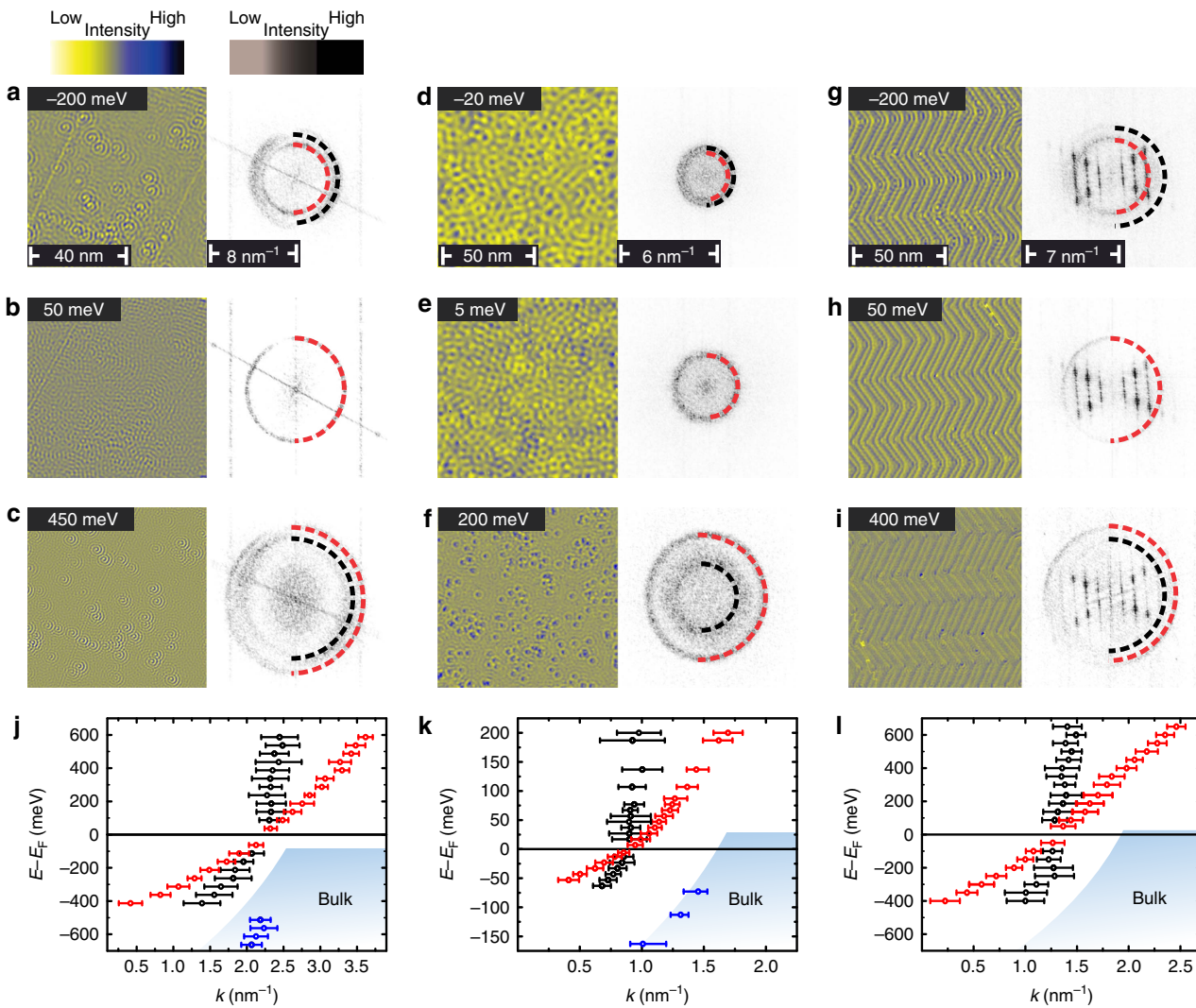
Figure 1 | Spectroscopic mapping of charge waves. (a–i) dI/dU maps with respective FT images obtained at different energies on Cu, Ag and Au. Two distinct rings in FT images merging into a single one at energies close to E_F are visible on all three surfaces. Low row shows energy-wavevector dispersion relations of two rings for (j) Cu, (k) Ag and (l) Au. Data have been obtained by analysing the FT QPI pattern at different energies. Red points correspond to the surface-state dispersion. Black points correspond to the additional oscillations with wavevector denoted as k_{EH} . Below the onset of the surface states, wavevectors corresponding to bulk states can be detected for Cu and Ag. The error bars have been calculated according to the procedure described in the Methods section.
