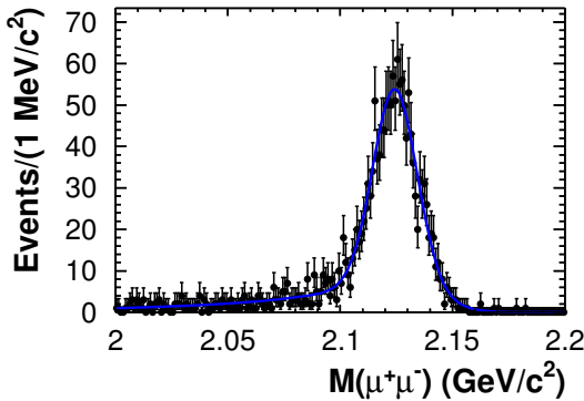
Fig. 4. Fit to M(\mu^+\mu^-) for run 42030. Dots with error bars are data, while the solid line is the fit result.
