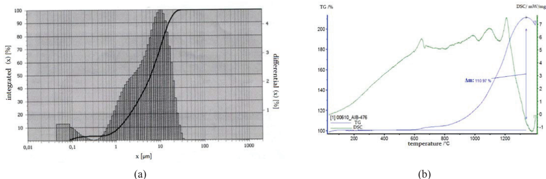
FIGURE 2. Particle size distribution (a) and DTA analysis data (b) for \text{AlB}_2 powder produced by means of SHS.
