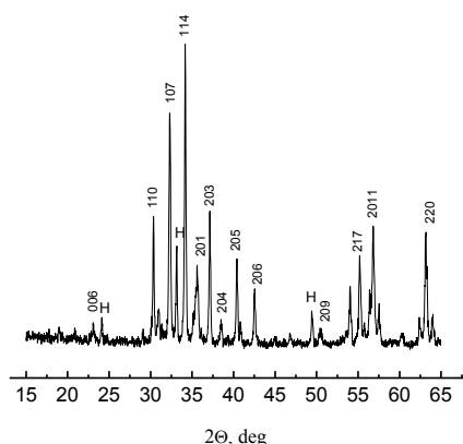
Figure 1. X-ray diffraction pattern of \text{SrFe}_{12}\text{O}_{19} hexaferrite powder synthesized by sol-gel combustion method. The letters H show the traces of the hematite phase.
