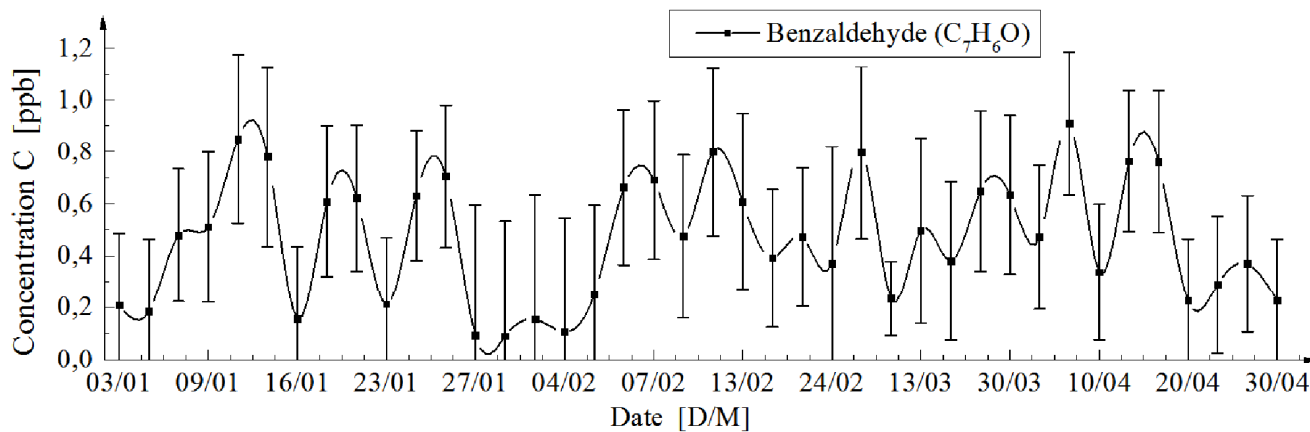
Fig. 8. Long-term variations of Benzaldehyde C_7H_6O concentration
