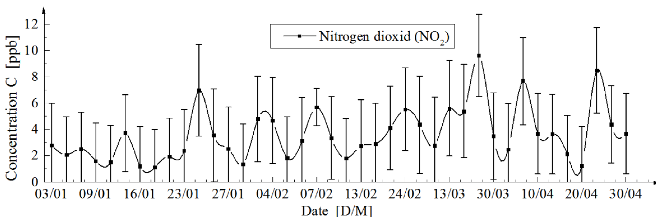
Fig. 4. Long-term variations of \text{NO}_2 concentration
