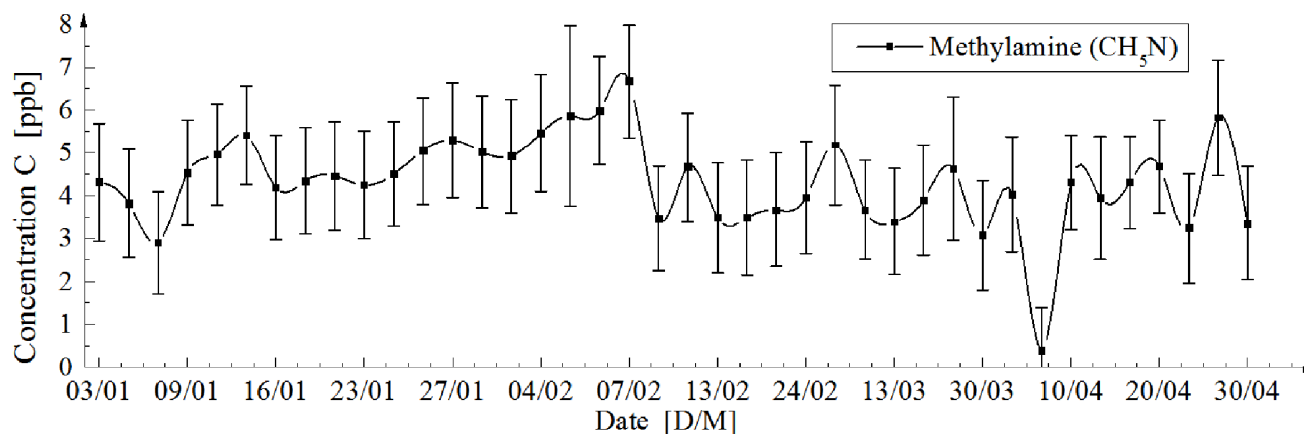
Fig. 5. Long-term variations of Methylamine \text{CH}_3\text{N} concentration
