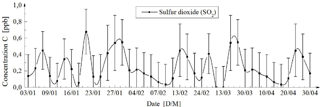
Fig. 3. Long-term variations of SO_2 concentration
