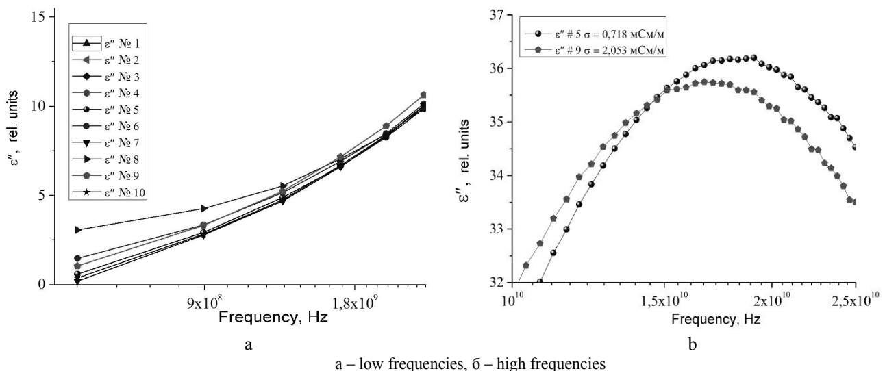
a – low frequencies, б – high frequencies Fig. 3. Permittivity of water samples of the second series. Temperature T = 23\text{ }^{\circ}\text{C}
