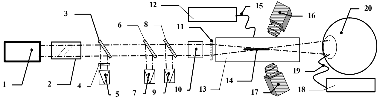
Fig. 1. Block diagram of the experimental setup comprising laser system 1 with \lambda_{01} = 800 nm, E_{01} = 1 mJ, \lambda_{02} = 400 nm, E_{02} = 0.3 mJ, pulse repetition frequency of 1 kHz, t_p = 35 fs, and d = 7 mm (Spitfire Pro 40F, Spectra Physics); compressor 2; rotating plates 3, 6, and 8; filter 4; PSCOUT PL-SP-LF autocorrelator (Spectra Physics) 5; 407A energy meter (Spectra Physics) 7; beam profiler 9; beta barium borate BBO ( \beta -BaB 2 O 4 ) conversion crystal 10 at 300 \mu m; removable focusing lens (BK7 plano-convex lens with d \sim 6 mm) 11 with f = 50.2 mm; Maya 2000Pro spectrometer 12; cell 13 with length L = 10 cm and thickness of the input window of 150 \mu m that was filled with water; filamentation region 14; optical waveguides 15 and 19; JVC GZ-MG255 video camera 16; SONY DSC-F828 camera 17; HR4000 spectrometer (Ocean Optics) 18; and integrating sphere 20.
