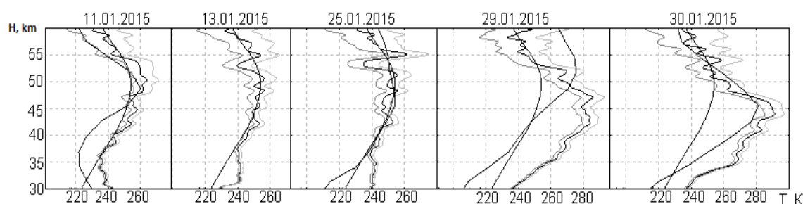
Figure 3. Vertical distribution of temperature in January 2015
