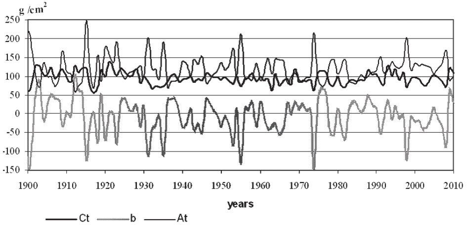
Fig. 3. Time course of the a, c, b in Malyi Aktru glacier
