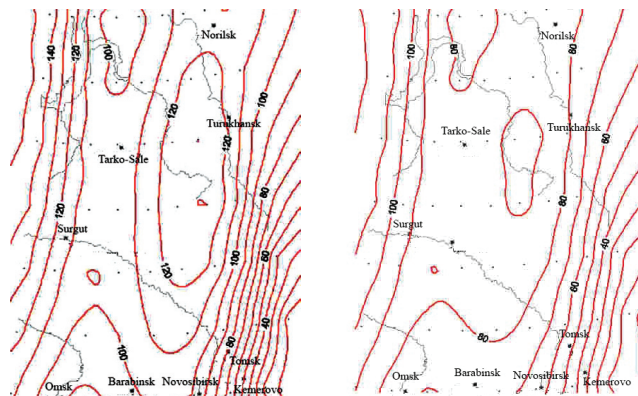
Fig 1. The distribution of average long-term number of cases with inversion in the layer 1000–925 hPa for night terms (00–06 h) during 1990–2010 years
